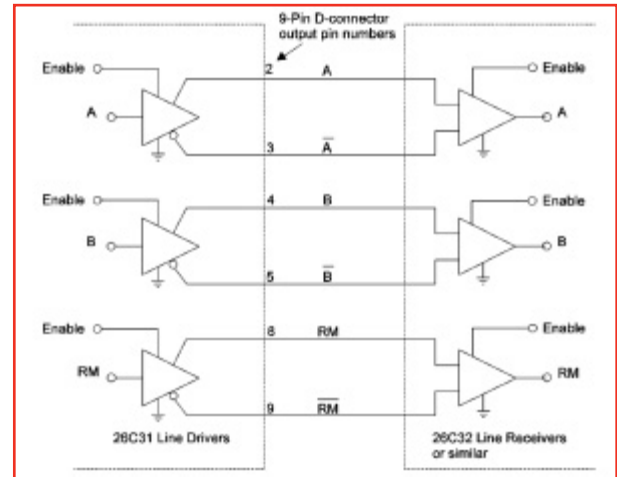
Encoder Connections
