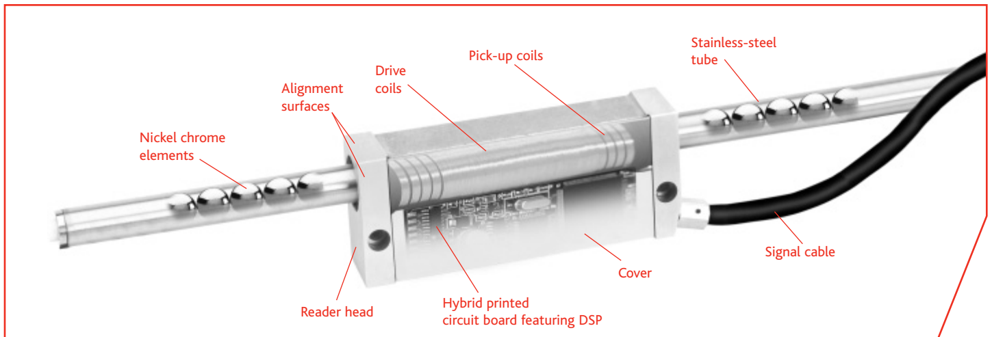
Sectional view
